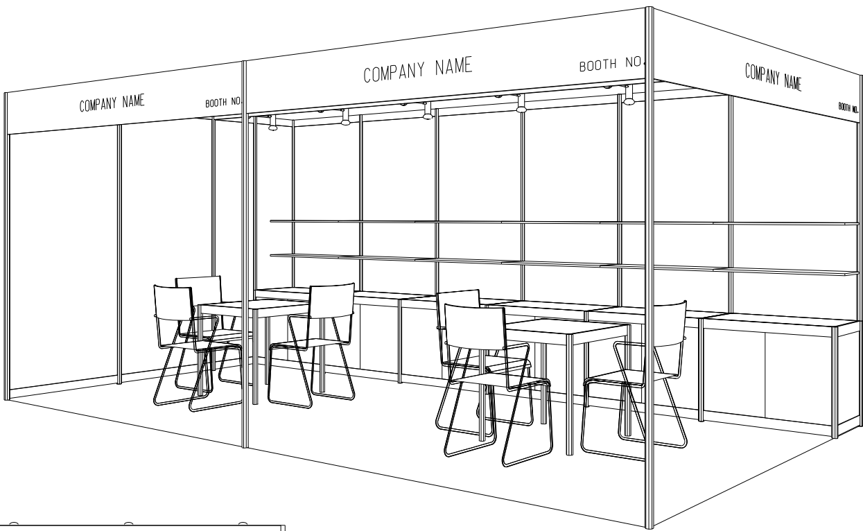
PERSPECTIVE 6M(W) X 3M(D) X 2.5M(H) Right Corner Booth A
