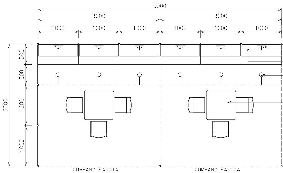
PLAN 6M(W) X 3M(D) X 2.5M(H) Right Corner Booth A
