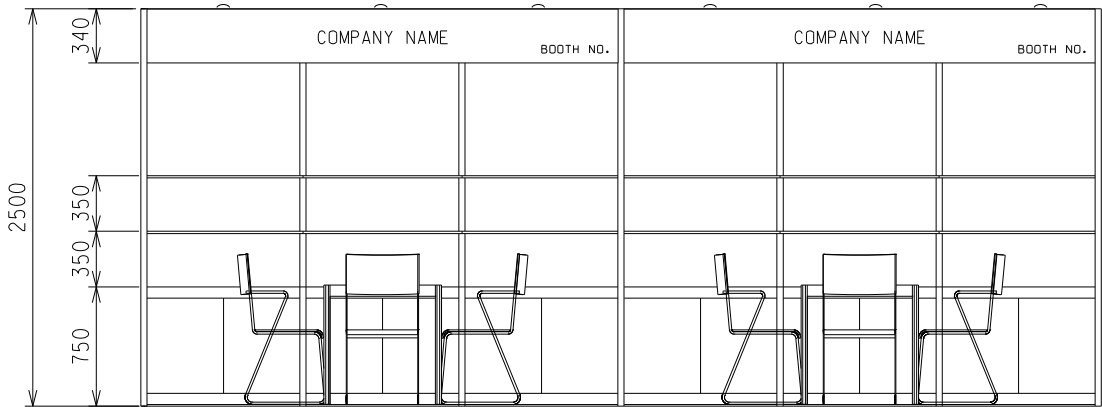
ELEVATION 6M(W) X 3M(D) X 2.5M(H) Right Corner Booth A
